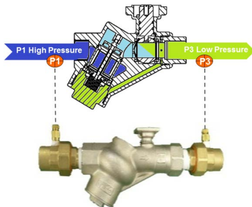
1" "Thru 2" PICCV - External PT Port Design
