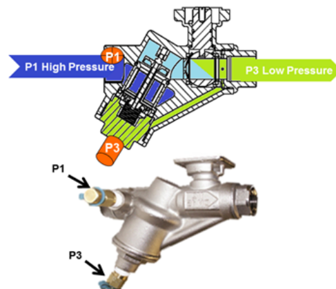
½" & ¾" PICCV - Integral PT Port Design
